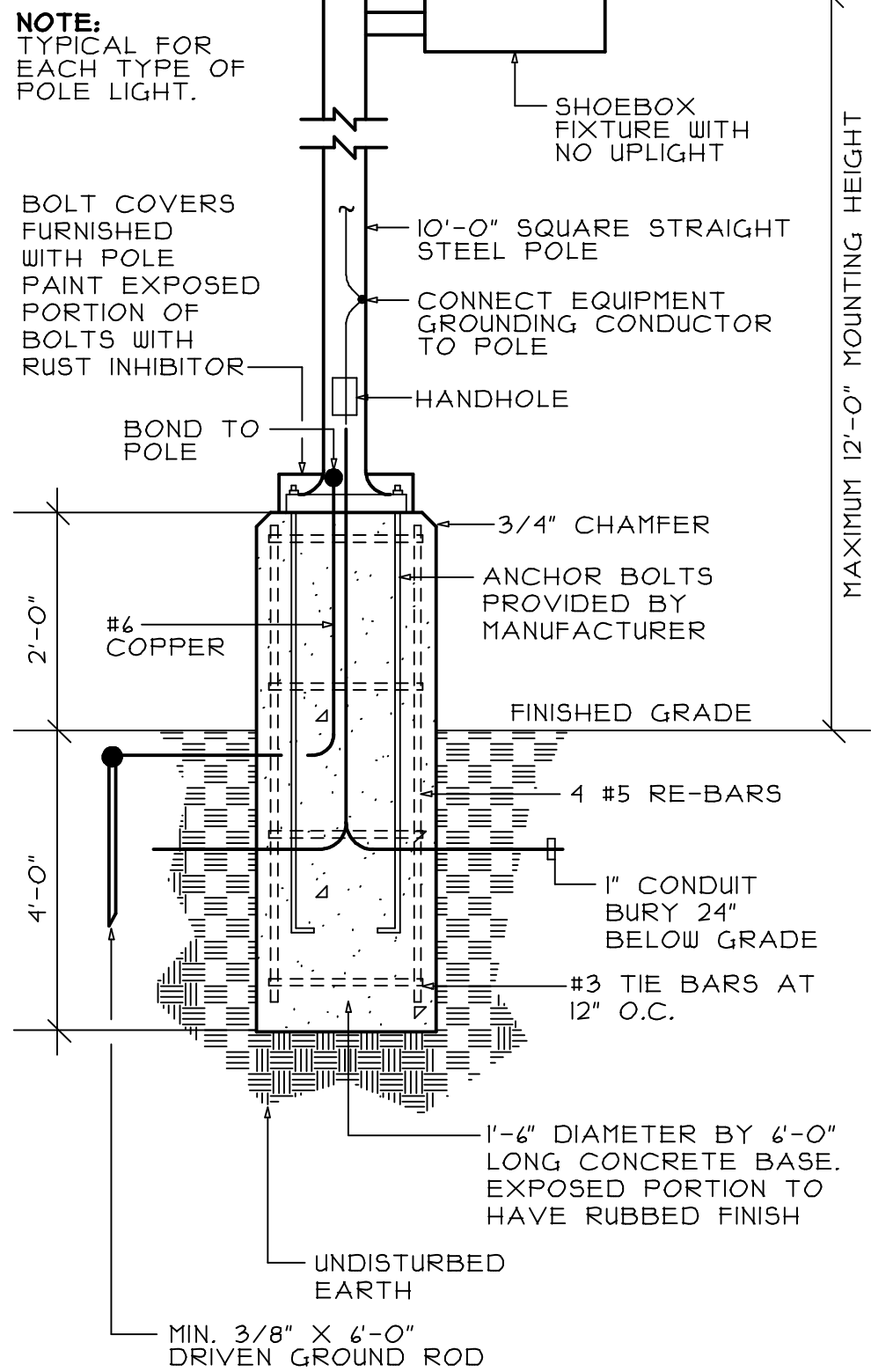
POLE BASE DETAIL NO SCALE
